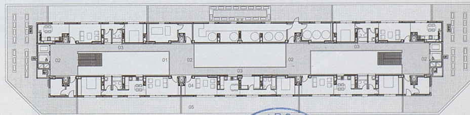
Plan Penthouses
