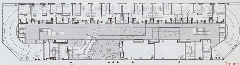
Ground Floor
